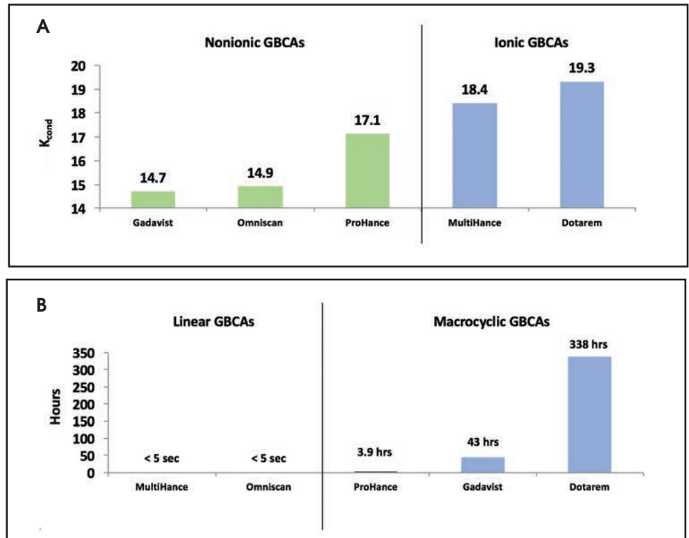
FIGURE 1. Conditional thermodynamic stability (A) and T_{1/2} (B) values for GBCAs. 8
